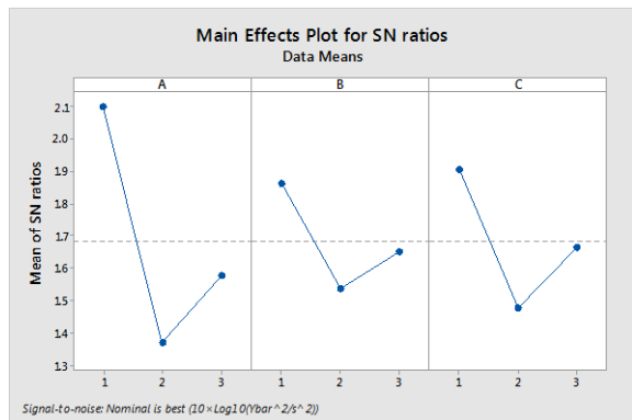
Fig. 4. Main Effects Plot for SN ratios
