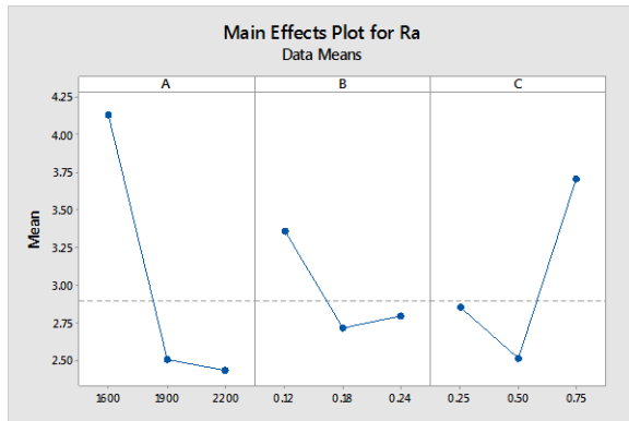
Fig. 3. Main Effects Plot for Means
