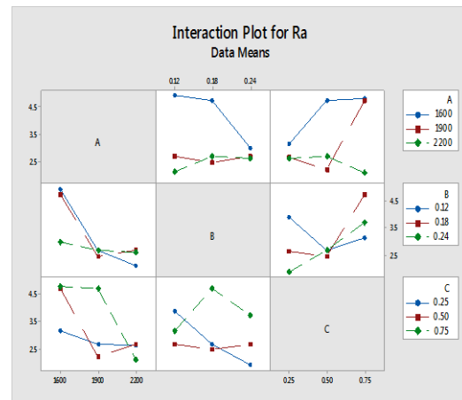
Fig: 2. Interaction Plot of Ra
