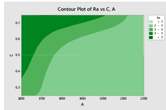
Fig. 6. Contour Plot of Ra vs C, A
