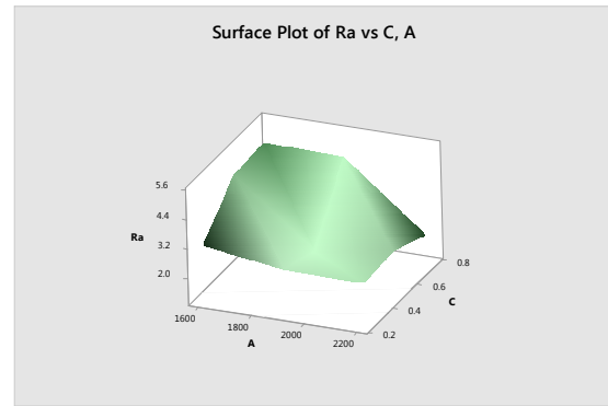
Fig. 5. Surface plot of Ra vs C, A
