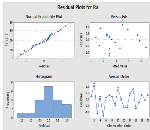
Fig: 1. Residual Plots for Ra
